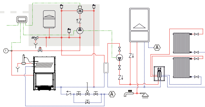
Kit camino-caldaia VC + centralina. Accessorio Hydrotherm 70V. VC Fireplace kit-boiler + control unit. 70V Hydrotherm accessory. Kit cheminée-chaudière VC + panneau de commande. Accessoire Hydrotherm 70V. Kit camino-caldaia VC + centralina. Accessorio Hydrotherm 70V. Kit chimenea-caldera VC + centralita. Accesorio Hydrotherm 70V.
