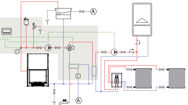
Kit camino-caldaia ACS-VA + centralina. Accessorio Hydrotherm. ACS-VA Fireplace kit-boiler + control unit. Hydrotherm accessory. Kit cheminée-chaudière ACS-VA + panneau de commande. Accessoire Hydrotherm. Bausatz Kamin-Kessel ACS-VA + Steuergerät. Zubehör Hydrotherm. Kit chimenea-caldera ACS-VA + centralita. Accesorio Hydrotherm.
