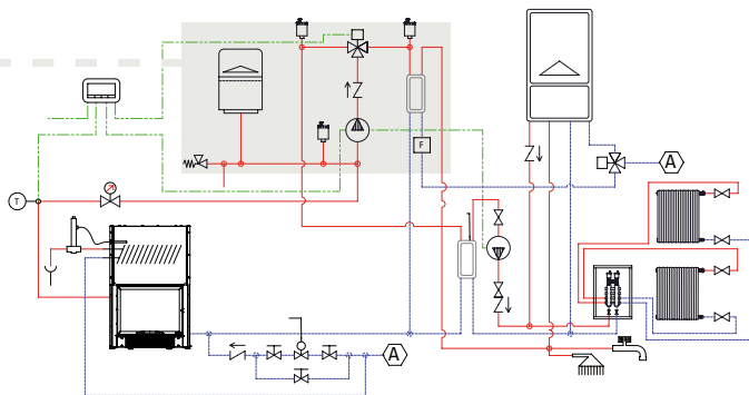
Kit camino-caldaia ACS-VC + centralina. Accessorio Hydrotherm 70V. ACS-VC Fireplace kit-boiler + control unit. 70V Hydrotherm accessory. Kit cheminée-chaudière ACS-VC + panneau de commande. Accessoire Hydrotherm 70V. Kit camino-caldaia ACS-VC + centralina. Accessorio Hydrotherm 70V. Kit chimenea-caldera ACS-VC + centralita. Accesorio Hydrotherm 70V.
